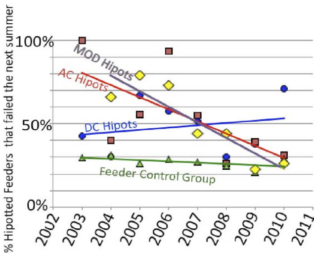
Fig. 23. Overtreatment in the High Potential Preventive Maintenance program was identified by comparing to control group performance. Modified and A/C Hipot tests are now used by Con Edison instead of DC Hipot tests.
