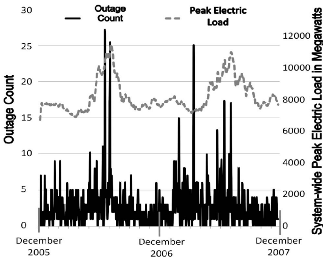
Fig. 2. Number of feeder outages in NYC per day during 2006-2007, lower curve with axis at left, and system-wide peak system load, upper curve with axis at right.
