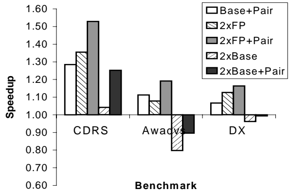
Figure 11: Relative performance of various processor models assuming that the register file access delay determines processor cycle time.
