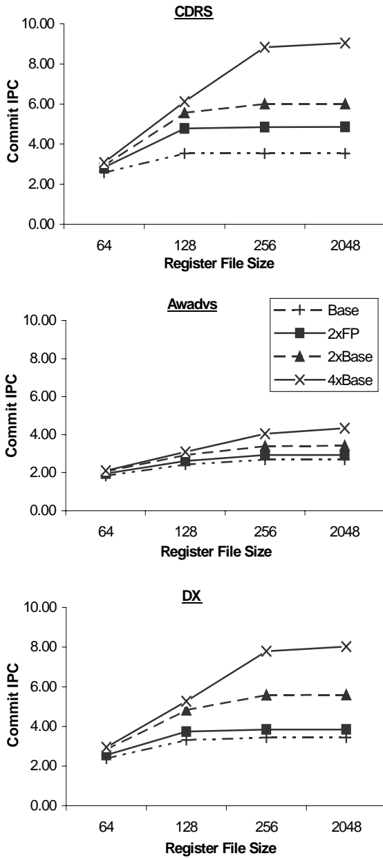
Figure 7: The commit IPC for various processor models with varying register file size.
