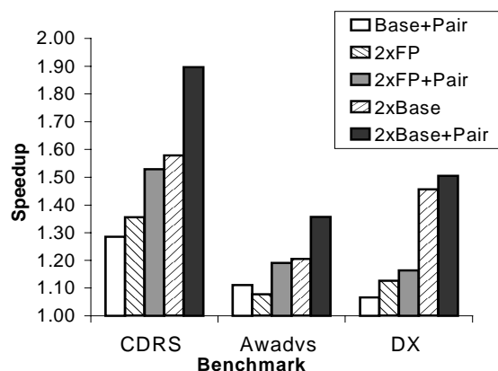
Figure 9: Relative speedup of various processor models over the Base with a dispatch queue of 64 entries and 128 registers.
