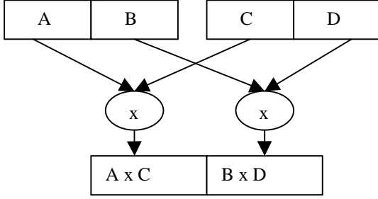
Figure 4: Operation of paired-single multiply.
