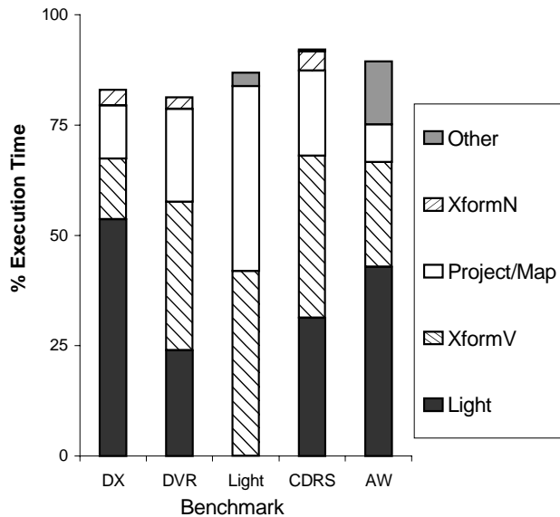
Figure 3— Execution time distribution in the MESA geometry pipeline.
