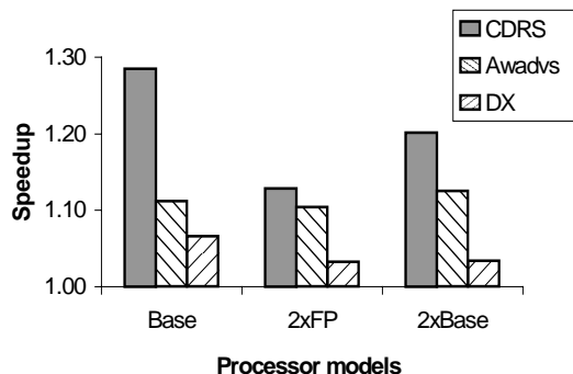
Figure 8: Performance improvement of paired-execution.
