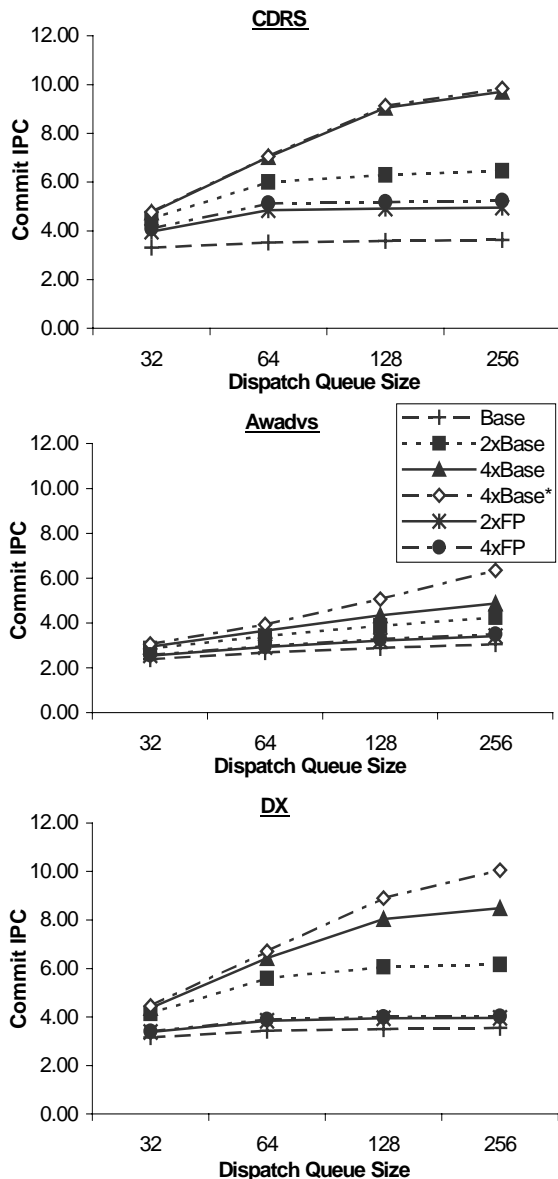
Figure 6: The commit IPC of various processor models with varying dispatch queue size. (4xBase* represents the issue IPC of the 4xBase processor)
