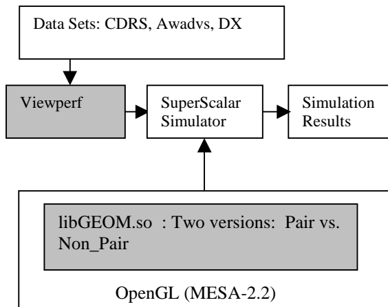
Figure 5: Simulation framework.
