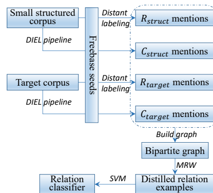
Figure 2: Architecture of DIEJOB.
