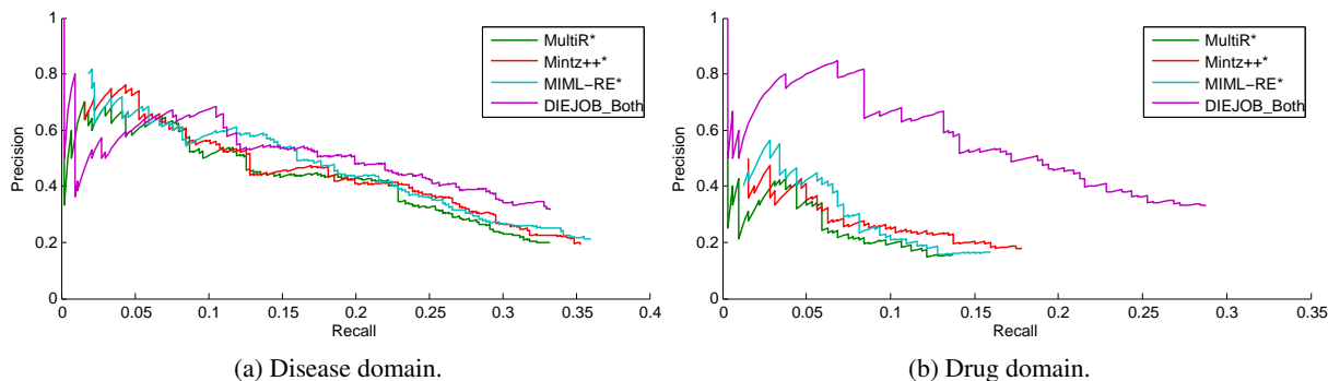
Figure 4: Precision-recall curves.
