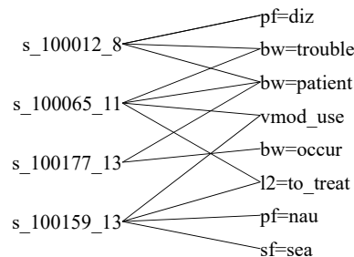
Figure 3: A bipartite graph of relation label propagation, with unique IDs on the left and features on the right (refer to Section 2.5).
