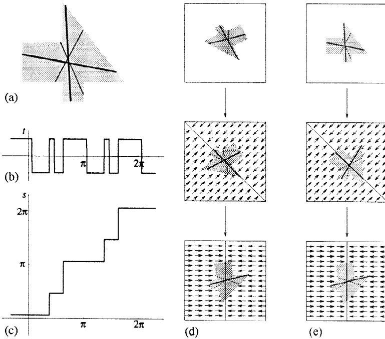
Fig. 10. (a) Polygonal part. Stable (thick line) and unstable (thin line) bisectors are also shown. (b) Moment function. (c) Turn function, which predicts the orientations of the stable and unstable bisectors. (d) Squeeze function, constructed from the turn function. (e) Alignment strategy for two arbitrary initial configurations.
