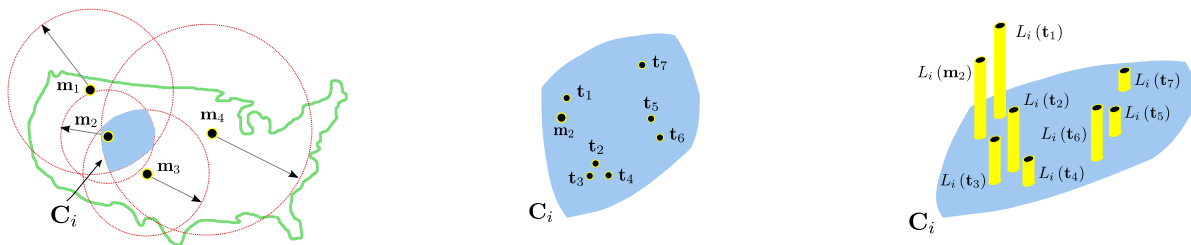
Figure 3: (Left) - Example construction of constrained geographic region C_i using observed latency from monitors \{m_1, m_2, m_3, m_4\} to target i . (Center) - Example set of constrained resources C_{R_i} , using monitors ( m_2 ) and landmarks ( \{t_1, \dots, t_7\} ) located inside the constrained region, C_i . (Right) - The estimated log-likelihood for each constrained resource location using Equation 3, with the estimated geographic location ( \hat{\mathbf{x}}_i = t_1 ) associated with the largest calculated log-likelihood value, L_i(t_1) .
