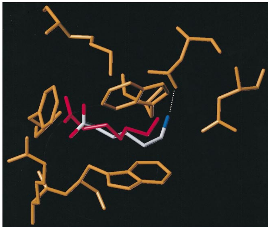
Figure 13. A section of the binding pocket of 2pk4 is shown together with the conformation of the ligand as found by X-ray crystallography (ranked as no. 129 by DrugScore, color-coded by atom type). The geometry of the best scored docking solution deviating by 1.3 Å from the crystal structure is depicted in red. In the crystal, the ligand forms a hydrogen bond between the terminal amino group and a carboxylate group of the protein that measures to only 2.1 Å length (shown as a dotted line).
