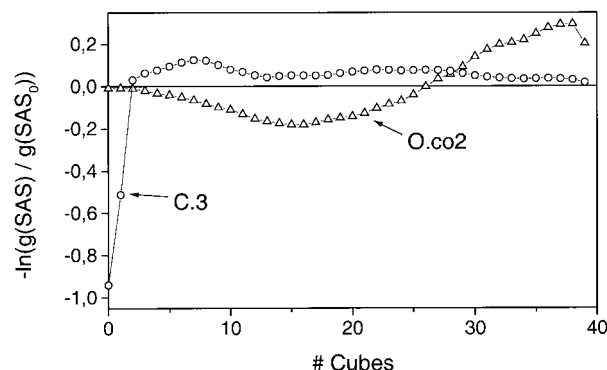
Figure 6. Statistical preferences for ligand atoms of type C.3 and O.co2 as calculated from the distribution functions for solvent accessibility of both atom types for complexed and separated state from the protein according to equation (7). The number of cubes (#cubes) is an approximate measure for the solvent accessibility; zero cubes refer to complete burial.
