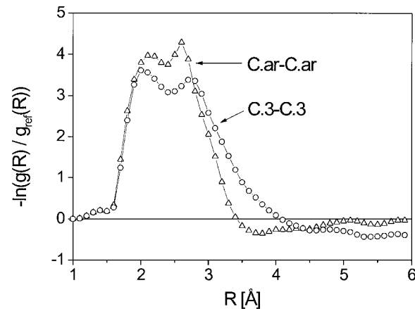
Figure 4. Statistical preferences for nonpolar/aromatic pair interactions as a function of the distance R , calculated according to equation (5).
