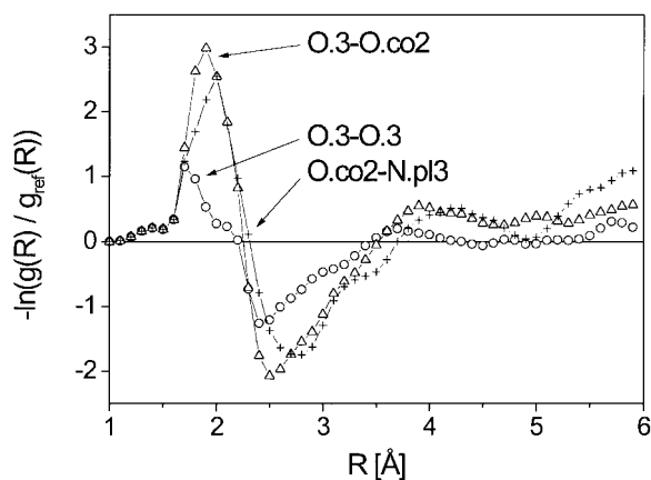
Figure 3. Statistical preferences for polar/charged pair interactions as a function of the distance R , calculated according to equation (5).
