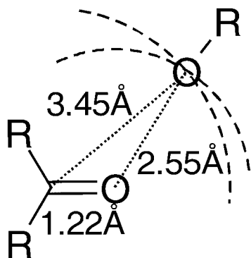
Figure 5. Intrinsic geometrical constraints reflected by the atom pair preferences of O.2-O.3 and C.2-O.3. Given the minima of the statistical pair preferences (O.2-O.3: 2.55 Å; C.2-O.3: 3.45 Å) and the bond length (C.2-O.2: 1.22 Å), the C.2-O.2-O.3 angle is calculated to be 128°.
