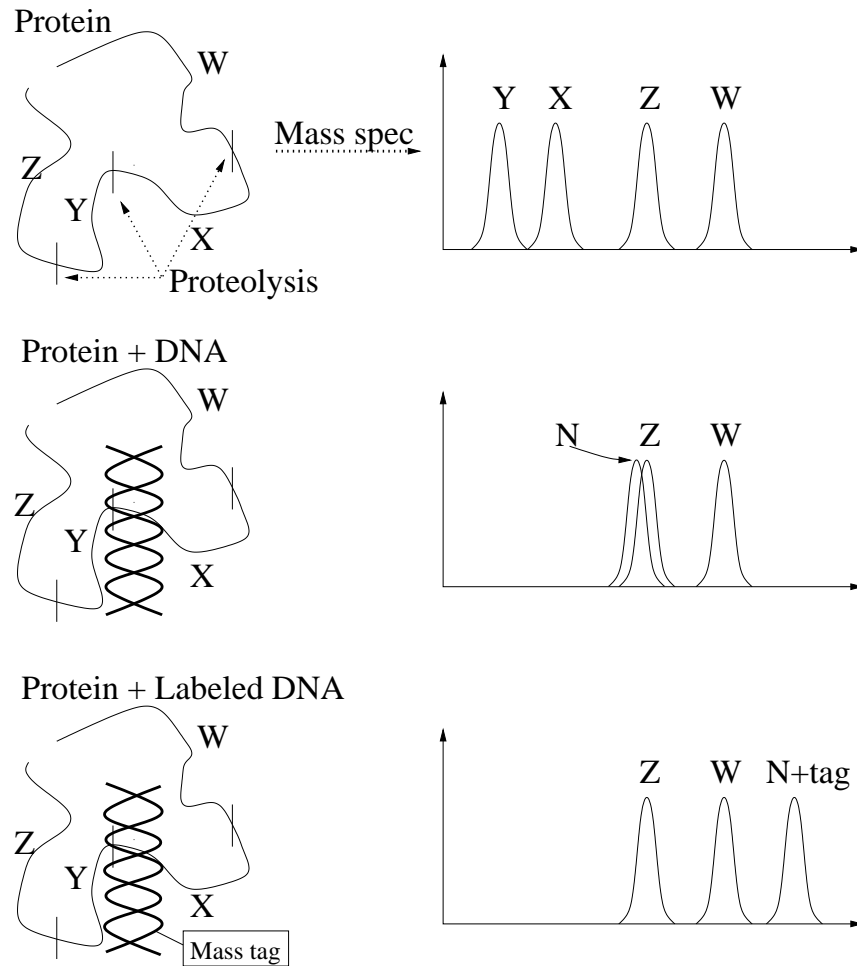
Figure 1: Mass tags can eliminate potential degeneracies in fragment hypotheses. (top) Proteolysis of an isolated protein yields four fragments, W, X, Y, and Z, with distinct masses. (middle) In the protein-DNA complex, the X/Y cleavage site is shielded, so that there are only three fragments, W, N, and Z, where N is the fragment X \cup Y complexed with the DNA. The mass of fragment N is very similar to that of fragment Z, yielding mass degeneracy. (bottom) Selective isotopic labeling is planned to ensure that the mass of fragment N+\text{tag} is distinguishable from that of fragment Z.
