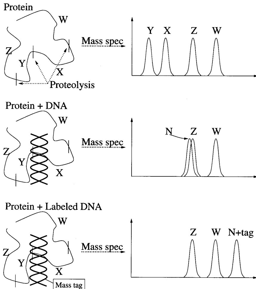
FIG. 1. Mass tags can eliminate potential degeneracies in fragment hypotheses. Proteolysis of an isolated protein yields four fragments, W, X, Y, and Z, with distinct masses ( top ). In the protein-DNA complex, the X/Y cleavage site is shielded, so that there are only three fragments, W, N, and Z, where N is the fragment X \cup Y complexed with the DNA. The mass of fragment N is very similar to that of fragment Z, yielding mass degeneracy ( middle ). Selective isotopic labeling is planned to ensure that the mass of fragment N+tag is distinguishable from that of fragment Z ( bottom ).
