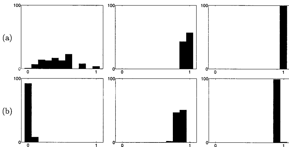
FIG. 3. Interpretability of randomly planned sets of 1, 2, and 5 labelings (left to right), for (a) UBL1 and (b) UBC9. Each bar indicates how many sets, out of 100, have the given probability of interpretability.
