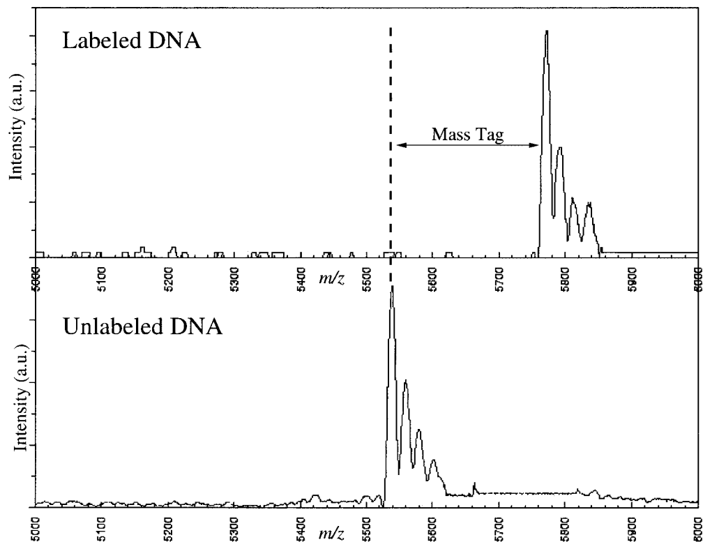
FIG. 2. MALDI-TOF mass spectra of an 18 bp DNA oligonucleotide d(GACATTGCGGTTAGGTC): ^{13}\text{C} -, ^{15}\text{N} -labeled 18-mer; ( top ) ^{12}\text{C} , ^{14}\text{N} -labeled 18-mer ( bottom ). The difference between the two peaks is called the mass tag.
