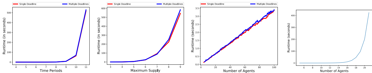
(a) The runtime for optimal solutions of variants with bounded charging speed and single or multiple deadline(s) (DP1) scales exponentially with the time horizon. (b) The runtime for optimal solutions of variants with bounded charging speed and single or multiple deadline(s) (DP1) scales exponentially with the maximum supply. (c) The runtime for optimal solutions of variants with bounded charging speed and single or multiple deadline(s) (DP1) scales linearly with the number of agents. (d) When demand and supply increase exponentially (i.e. for n agents, max supply is 2^n ), DP2 can solve instances up to 20 agents within 5 minutes.
