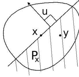
Fig. 2. Intuition behind Lemma 1. Consider the hyperplane normal to \mathbf{u} through \mathbf{x} . On one side of this hyperplane is \mathbb{P}_x , and for any \mathbf{y} in the region \mathbb{P}_x , G(\mathbf{x}) \geq G(\mathbf{y}) . By continuity of G , G(\mathbf{x}) must be constant along the hyperplane (the boundary of \mathbb{P}_x ).
