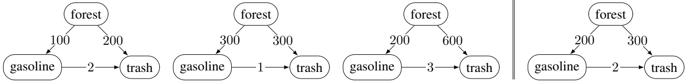
Figure 1: Example from Conitzer, Brill, and Freeman (2015) that illustrates that taking the median on each edge can lead to inconsistent outcomes even when each individual voter is consistent. Each of the left three graphs illustrates the consistent preferences of a single voter, with the label on each edge indicating the voters ideal tradeoff between the corresponding two activities. The rightmost graph, which results from taking the median on each edge, is inconsistent because 300 \neq 2 \cdot 200 .
