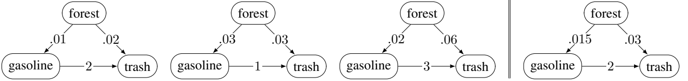
Figure 3: Example illustrating that a change of units can change the outcome on an unrelated edge under \text{DBR}^{\text{linear}} . The leftmost three graphs are the votes and the rightmost one is the outcome produced by \text{DBR}^{\text{linear}} .
