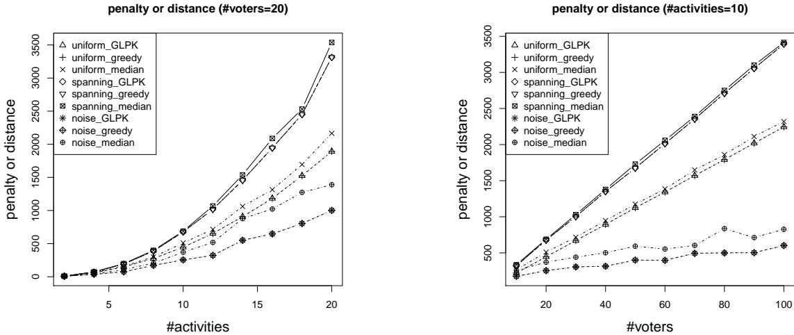
Figure 6: Performance comparison for different algorithms and distributions over vote profiles. “Penalty” is the sum of disagreement between the aggregated tradeoff and all votes (our LP objective): \sum_{i \in N} \sum_{(a,b) \in E} |\log(t^{ab}) - \log(t_i^{ab})| . For the noise case, we use distance to the ground truth instead of penalty. “Distance” is n \cdot |(q_a - q_b) - \log(t_i^{ab})| where q is the ground truth (after the log adjustment). We multiply the difference by the number of voters n so that it has the same scale as penalty.
