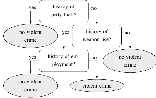
Figure 1: Decision tree induced by a SLIM model.
