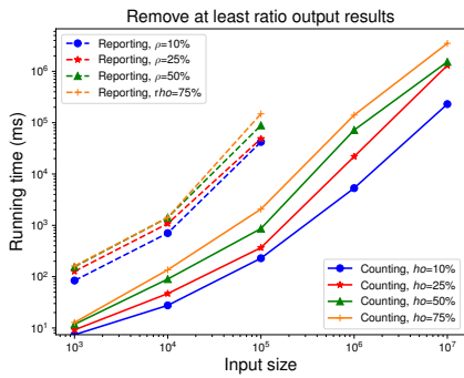
Figure 7: Running Time: \sigma_\theta Q_1 (easy) exactly (count/report).
