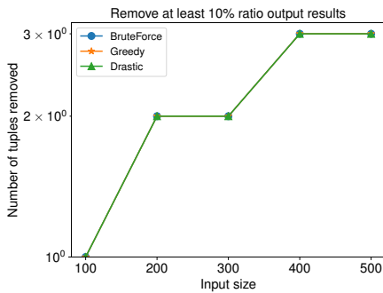
Figure 13: Quality: brute-force v.s. heuristics for Q_1 (hard).
