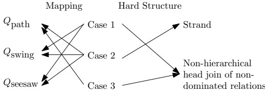
Figure 6: Correspondence between the three cases of hard query on which IsPTIME falling into “other” bucket in Figure 4, the core query it maps to (the left) and the hard structure it contains (the right).
