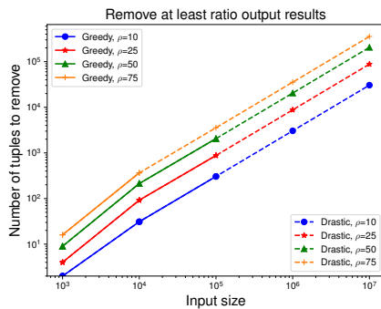
Figure 11: Quality: Q_1 (hard) by heuristics.
