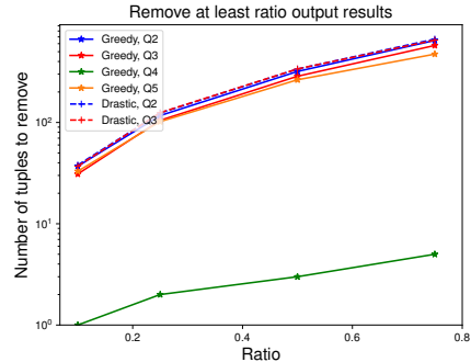
Figure 15: Quality: Q_2, Q_3, Q_4, Q_5 (hard) by heuristics.
