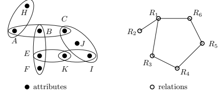
Figure 2: Hypergraph (left) and graph (right) representation for an example CQ Q(A, C, F, K) : -R_1(A, B, C), R_2(A, H), R_3(B, E, F), R_4(E, K), R_5(K, I), R_6(C, I, J) .
