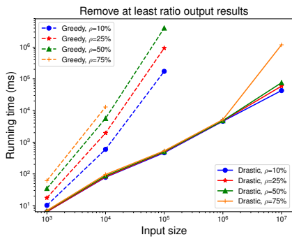
Figure 10: Running Time: reporting Q_1 (hard) by heuristics.
