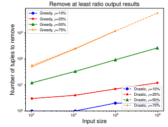
Figure 19: \alpha = 1 (hard)
