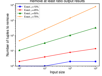
Figure 23: \alpha = 1 (easy)
