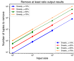
Figure 17: \alpha = 0 (hard)
