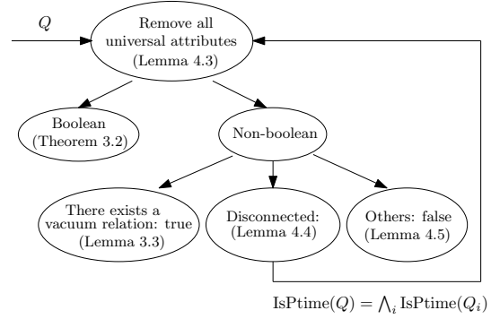
Figure 3: Procedure ISPTIME(Q) .
