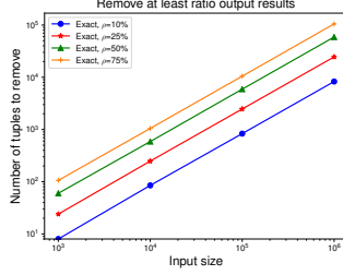
Figure 21: \alpha = 0 (easy)
