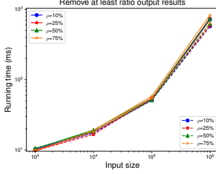
Figure 20: \alpha = 0 (easy)
