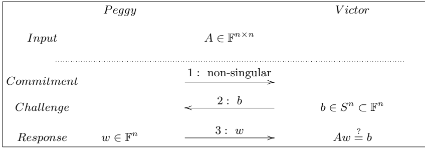
Figure 2: Blackbox interactive certificate of non-singularity
