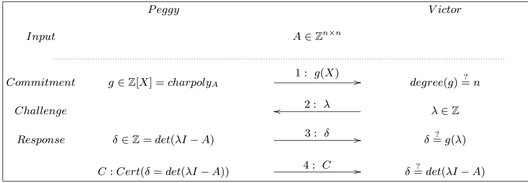
Figure 1: Interactive certificate for the characteristic polynomial
