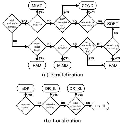
Figure 10: Decision trees for choosing mapping variant based on application characteristics. Note that MIMD is not strictly required in the decision, and its additional hardware requirements provide only up to 12% performance benefits.
