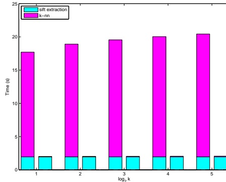
Figure 6: Speedup in SIFT feature matching by the parallel execution of TBiS on the GPU (the nearly invisible magenta bar to the right) over the serial execution of the k NN search procedure in VLFeat on a single-core CPU (the magenta bar to the left), for 1,024 queries into 65,536 corpus feature vectors of 128 dimensions and 32 neighbors. The light blue bars are the time for feature extraction on the single-core CPU.
