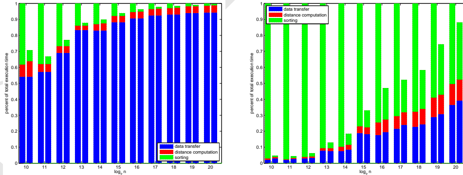
Figure 4: Performance profile in percentile for a single query (left) and 128 queries (right), respectively, data transportation in blue, distance calculation in red and neighbor location in green.
