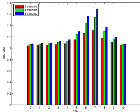
Figure 5: Further improvement with 2, 4 and 8 streams over a single stream when processing large and high-dimensional corpus (16, 777, 216 vectors of 128 dimensions).
