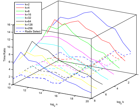
Figure 2: Comparison of TBiS and the MGPU radix-select for k NN search.
