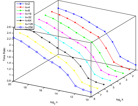
Figure 3: Improved k NN search by TBiS with the distance calculation and truncated sorting interleaved.
