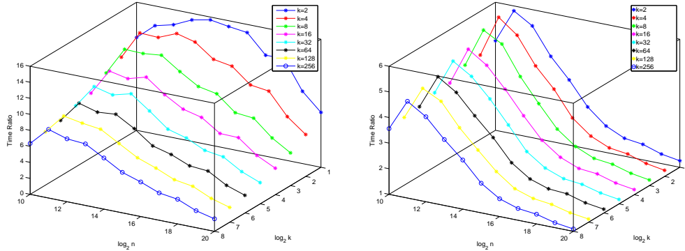
Figure 1: Comparison between two approaches : truncation after sort and truncation during sort, without distance evaluation (left) or with distance evaluation (right) but without interleaved with sorting.
