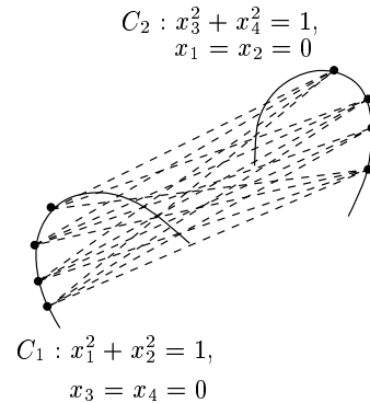
Figure 1: A construction for f_1^{(4)}(n) = \Omega(n^2) .
