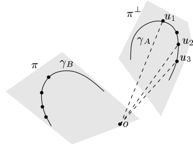
Figure 3: Illustration to the upper bound.
