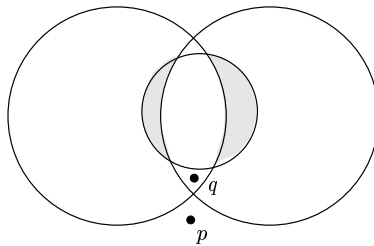
Figure 2: K_q \setminus K_p (the shaded region) consists of two connected components.
