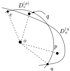
Figure 3: Proof of Theorem 2.6.
