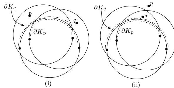
Figure 6: Counter-examples for Theorem 2.8 if we just consider intersection points (including noncrossings).
