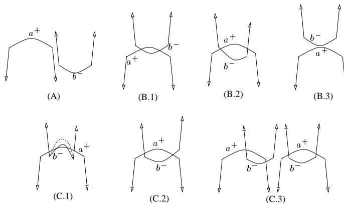
Figure 19. An extended upper arc and an extended lower arc intersect at most twice: (A) \rho_a lies to the left of \lambda_b ; (B) \lambda_b lies above a^+ : (B.1) a^+, b^- intersect at two points; (B.2) a^+ and b^- intersect at one point; (B.3) a^+ and b^- do not intersect. (C) \lambda_b lies below a^+ : (C.1) a^+ and b^- intersect at two points (an impossible configuration); (C.2) a^+ and b^- intersect at one point; (C.3) a^+ and b^- do not intersect.
