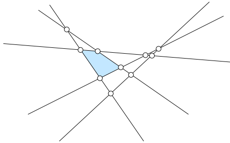
Figure 1: An arrangement of lines.
