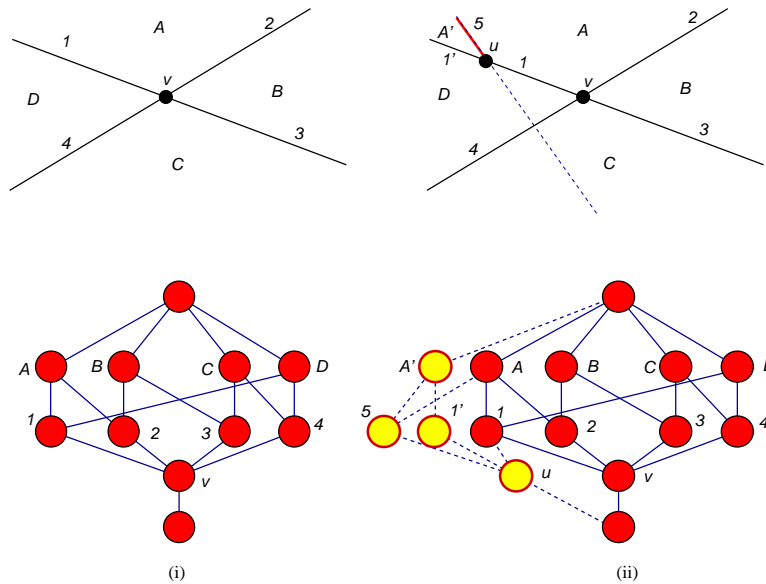
Figure 11: (i) Incidence graph of the arrangement of 2 lines. (ii) Adding a new line; incremental changes in the incidence graph as the vertex v , the edge 5, and the face A' are added.
