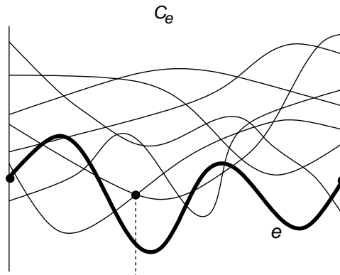
Figure 3: Vertical cylinder C_e and the vertical cross-section \Gamma_e of \Gamma .
