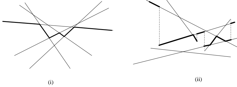
Figure 7: The 2-level in (i) an arrangement of lines, and (ii) in an arrangement of segments.
