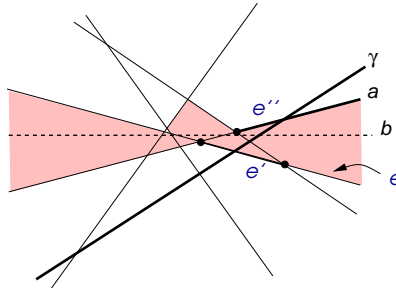
Figure 6: Inserting \gamma into zone(b; \Gamma \setminus \{\gamma\}) .
