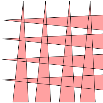
Figure 9: Union of Jordan regions.
