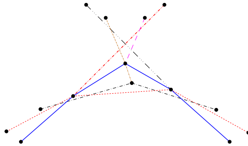
Figure 8: A set of 14 points with 14 halving segments, split into 7 convex x -monotone chains.
