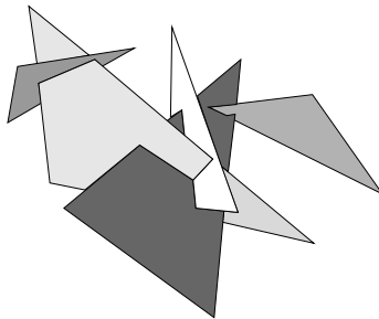
Figure 2: Lower envelope of triangles in \mathbb{R}^3 , as viewed from below.
