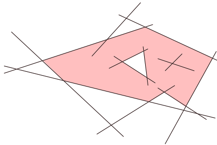
Figure 5: A single cell in an arrangement of segments.
