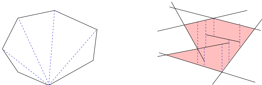
Figure 10: (i) Bottom vertex triangulation of a convex polygon; (ii) vertical decomposition of a cell in an arrangement of segments.
