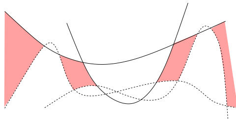
Figure 4: \mathcal{S}(\Gamma, \Gamma') ; solid arcs are in \Gamma , and dashed arcs are in \Gamma' .
