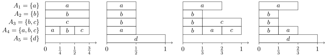
Figure 1: Illustration of Examples 2 and 3. From left to right: The first diagram illustrates a load distribution minimizing the maximal voter load \max_{i \in N} \bar{x}_i ; the second diagram illustrates the unique load distribution minimizing \sum_{i \in N} \bar{x}_i^2 ; the third and fourth diagrams illustrate the load distributions obtained by seq-Phragmén with ties broken in favor of c or d , respectively.
