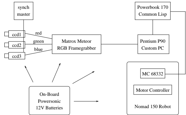
Figure 3: Architecture of the mobile robot.
