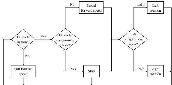
Figure 1: Robot control flowchart.
