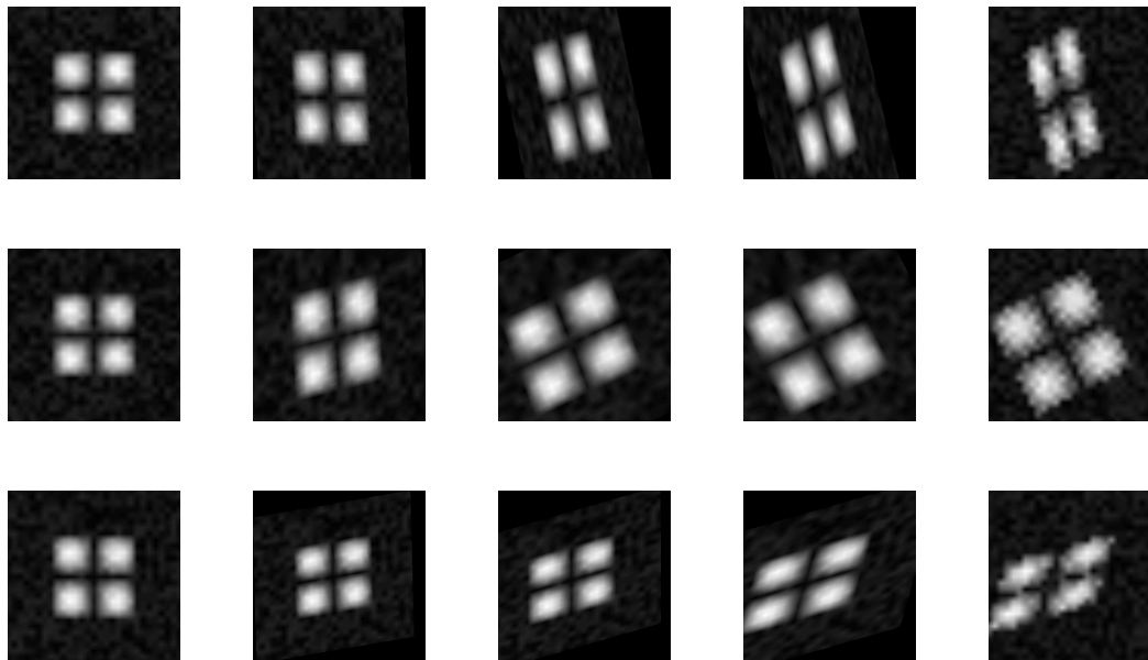
Figure 6.1: Original image (leftmost column) and image warped, translated and corrupted by noise (rightmost images) for three different motions. The intermediate columns are the images in the leftmost column deformed and translated by 4,8,and 19 iterations of the tracking algorithm.
