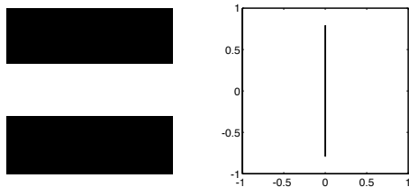
Figure 4.1: An image window with a white horizontal bar (left) and the corresponding confidence ellipse (right).
