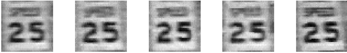
Figure 5.4: The same windows as in figure 5.2, warped by the computed deformation matrices.
